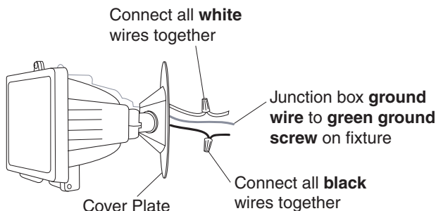
Wiring Fixture
